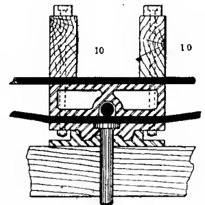
Fig. 1938. Section of Center-plate and Bolster-casting.
